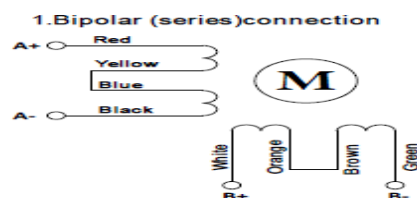
8-lead motor series connections
